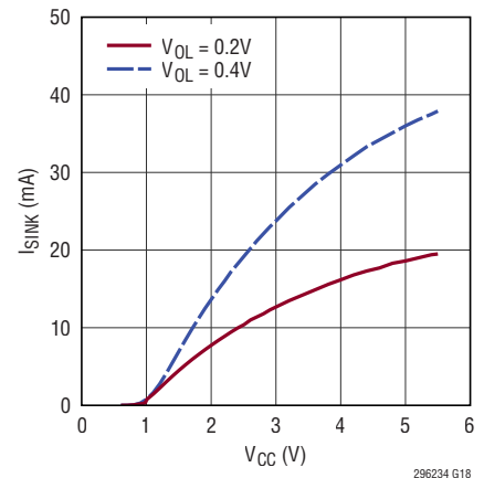
Output Logic Low, I_{SINK} vs V_{CC} \overline{RST} , \overline{WDO} , OUT_n
