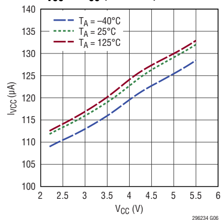
I_{VCC} vs V_{CC} (LTC2964)
